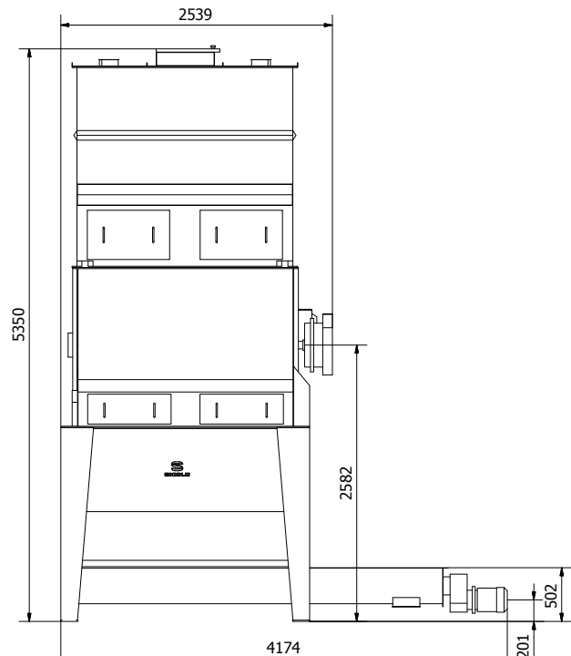
3-step - mixer + pre-bin + discharge bin
